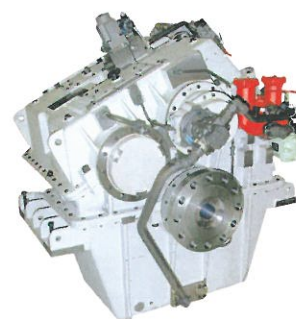
Reduction gearbox with built-in clutch, vertically offset
